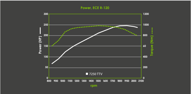
Greater torque reserve and more torque at lower engine speeds.
