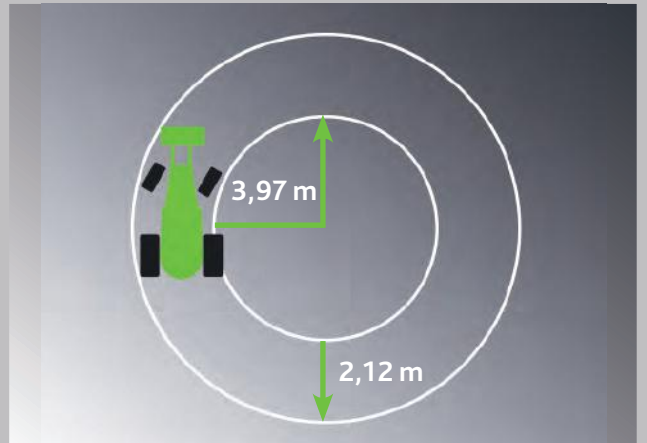
A turning circle of 3.97 m allows easy manoeuvring even in the tightest of spaces (depending on tyres and surroundings).
